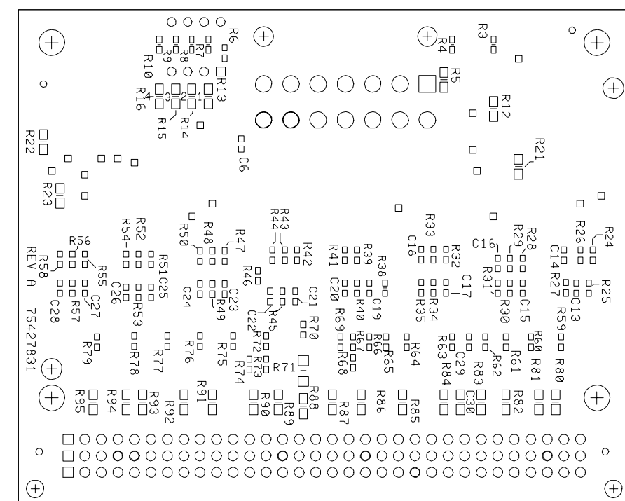
PRIMARY SIDE
