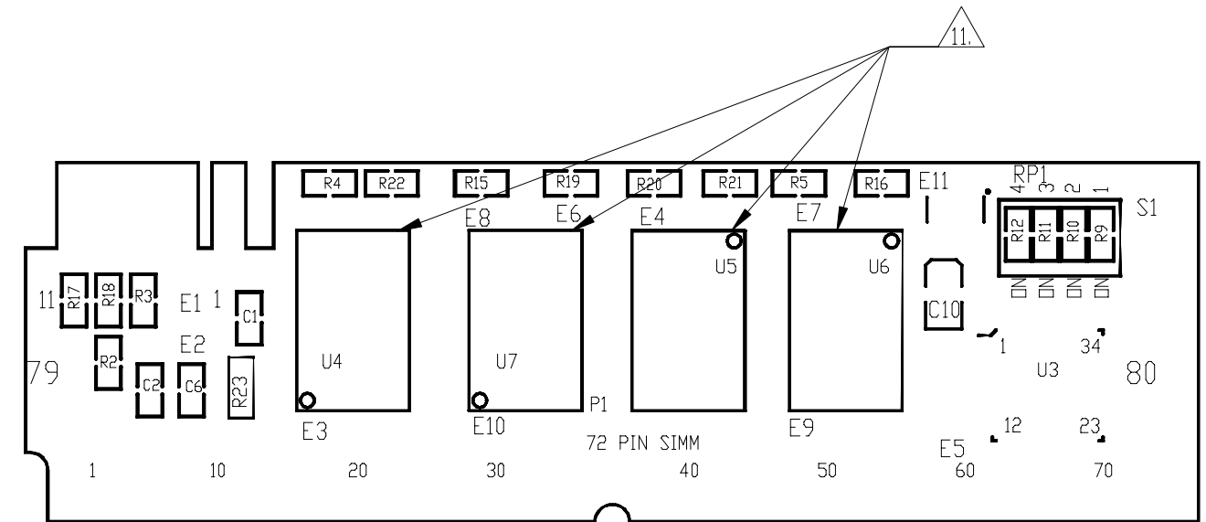
PRIMARY SIDE
