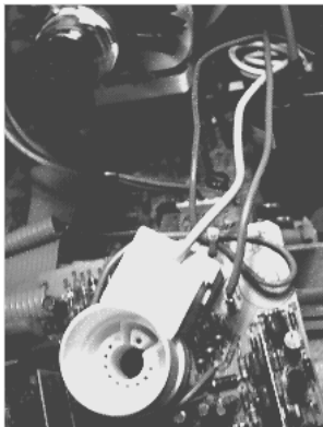
Route G2 wire around CRT socket, shorten with loop, and add wire tie.
