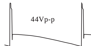
Vertical yoke drive, voltage waveform.
