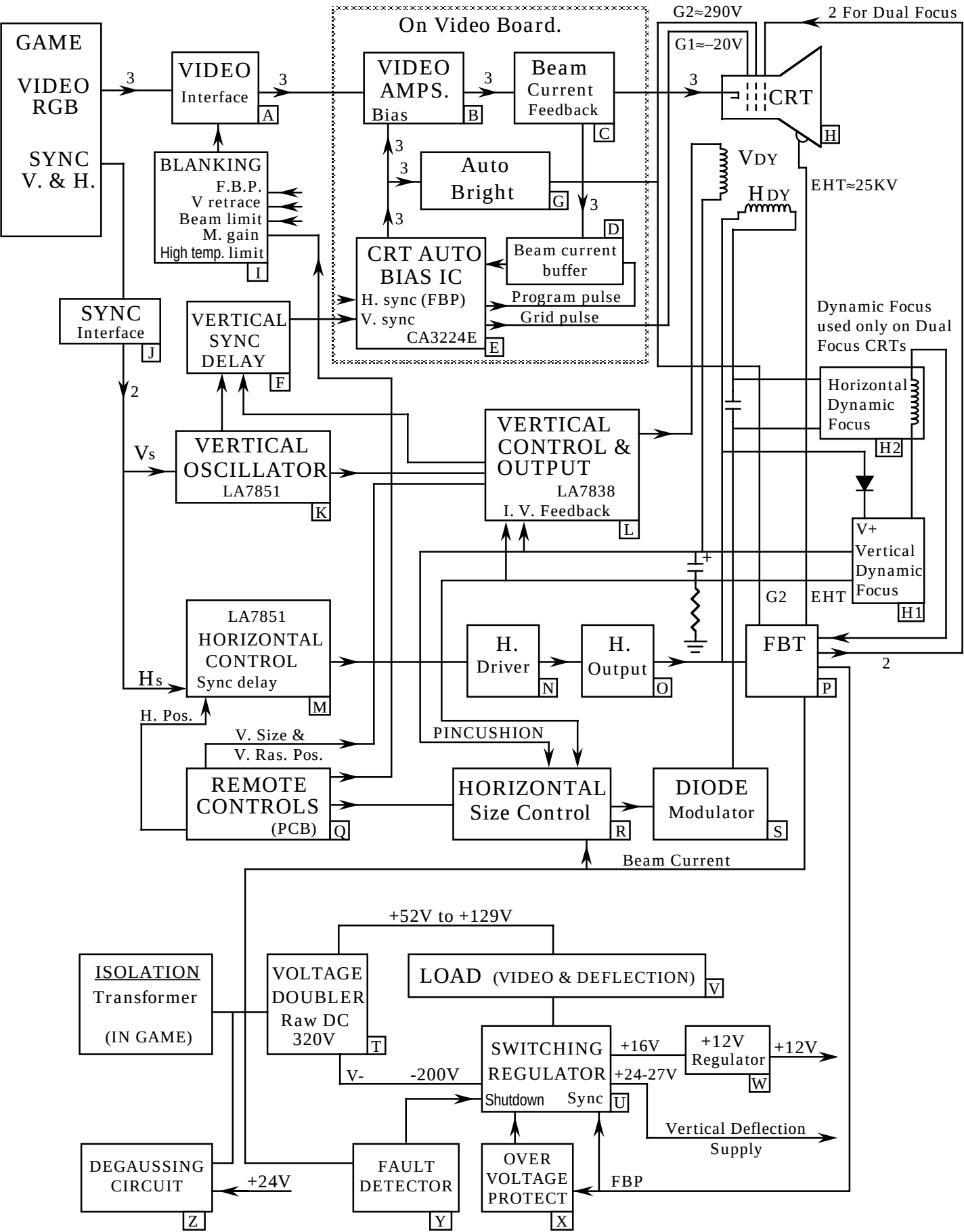
XX93 Monitor Block Diagram.
