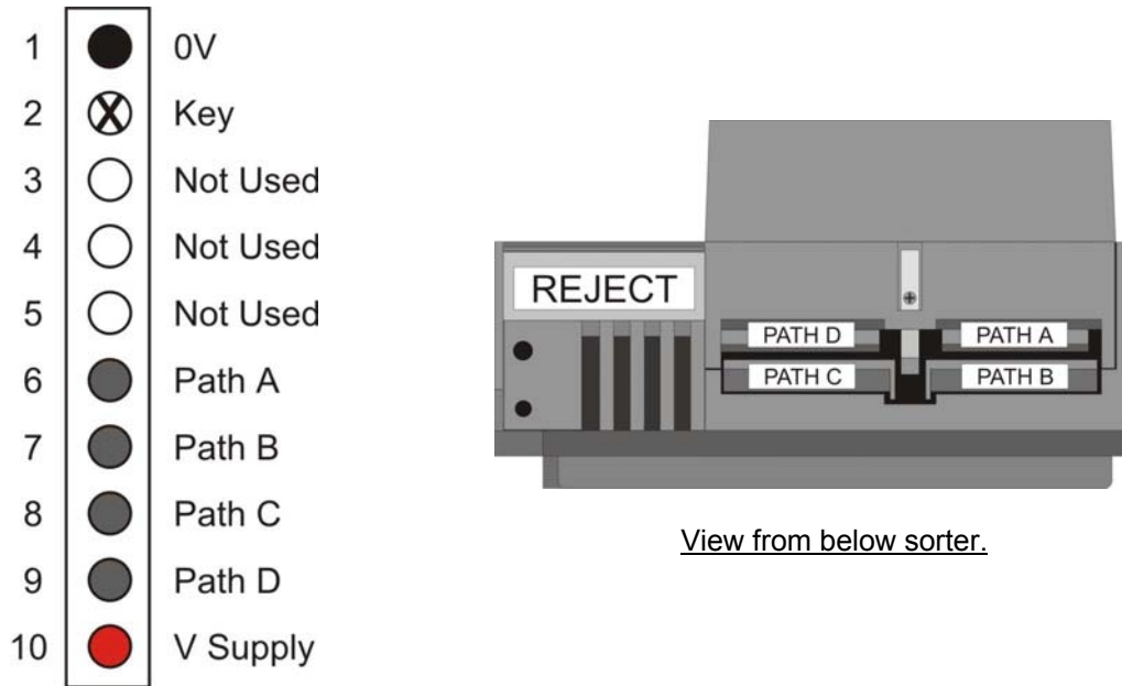
Figure 9: Sorter Overrides 4-way
