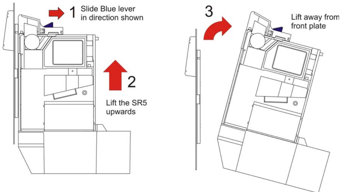
Figure 21: Front Entry Removal Diagram
