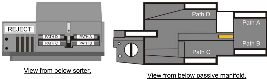
Figure 7: 4-way sorter paths
