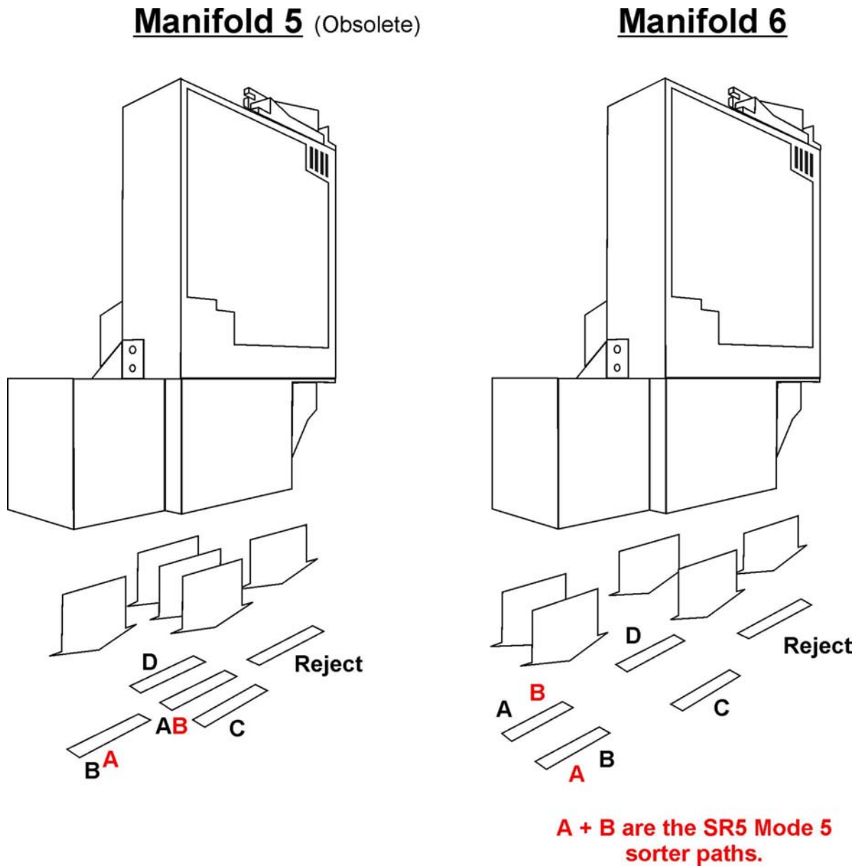
Figure 27: SR5 Manifold Coin Exit Paths
