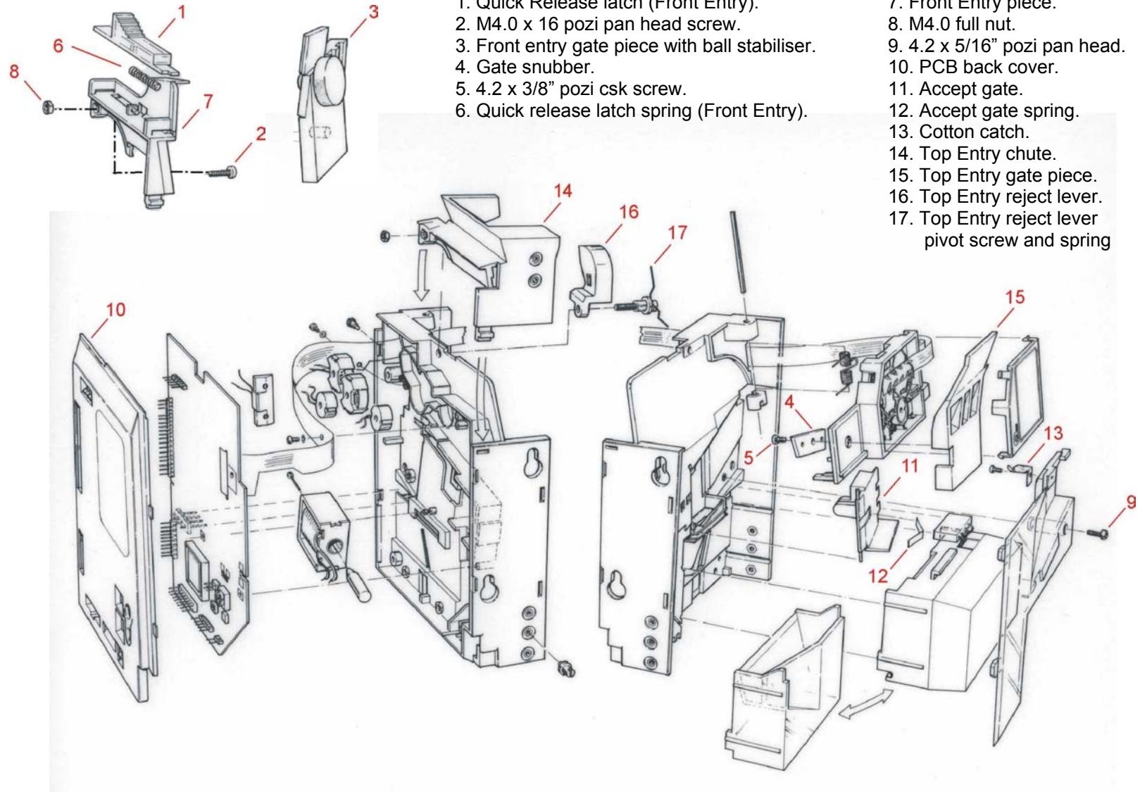
Figure 28: Top Entry / Front Entry Exploded View
