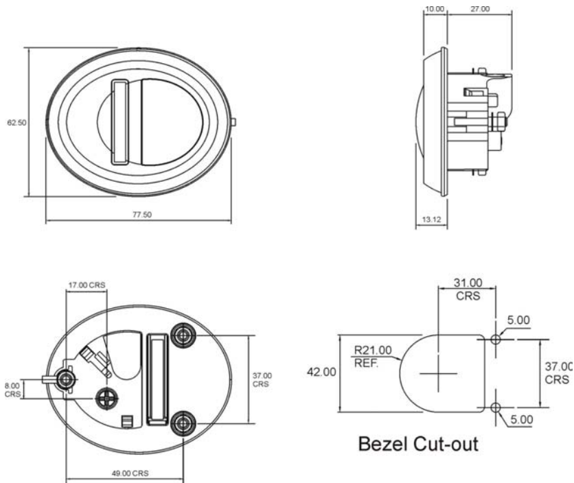
Figure 24: Oval Bezel Dimensions
