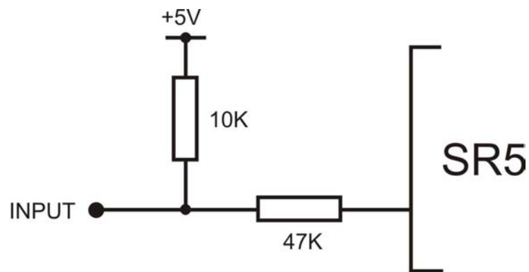
Figure 4: Input Hardware Configuration
