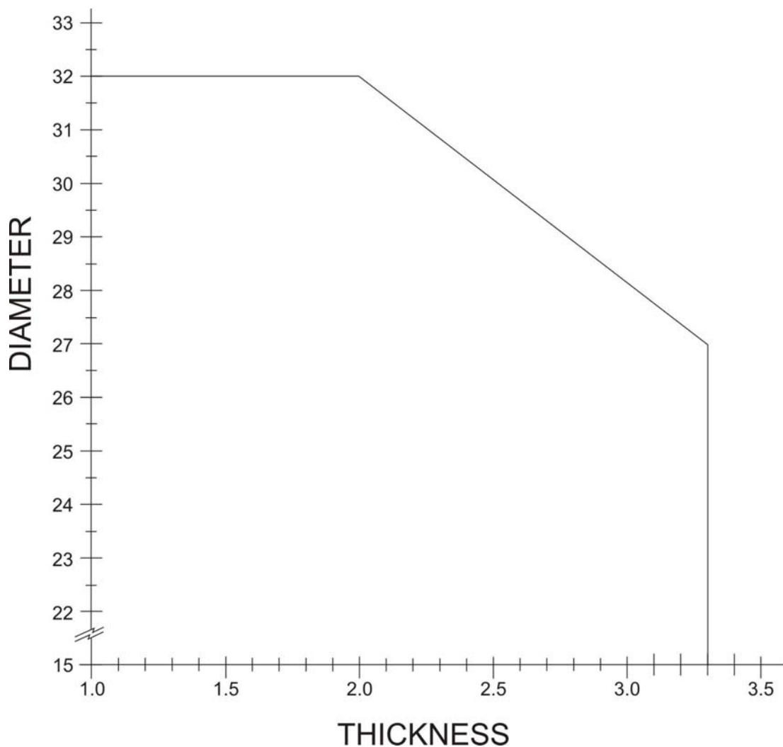
Figure 22: SR5 Accepted Coin Dimensions Graph
