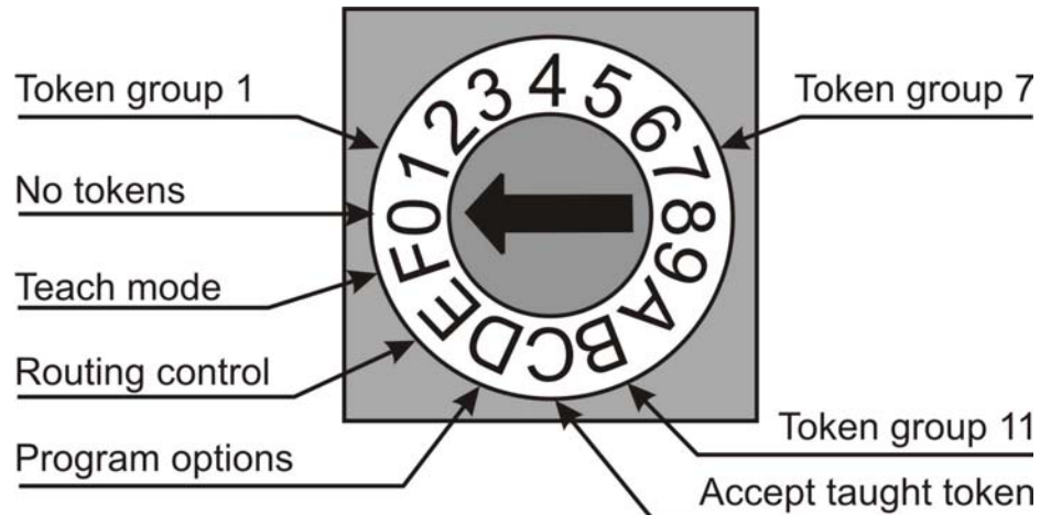
Figure 14: Rotary switch
