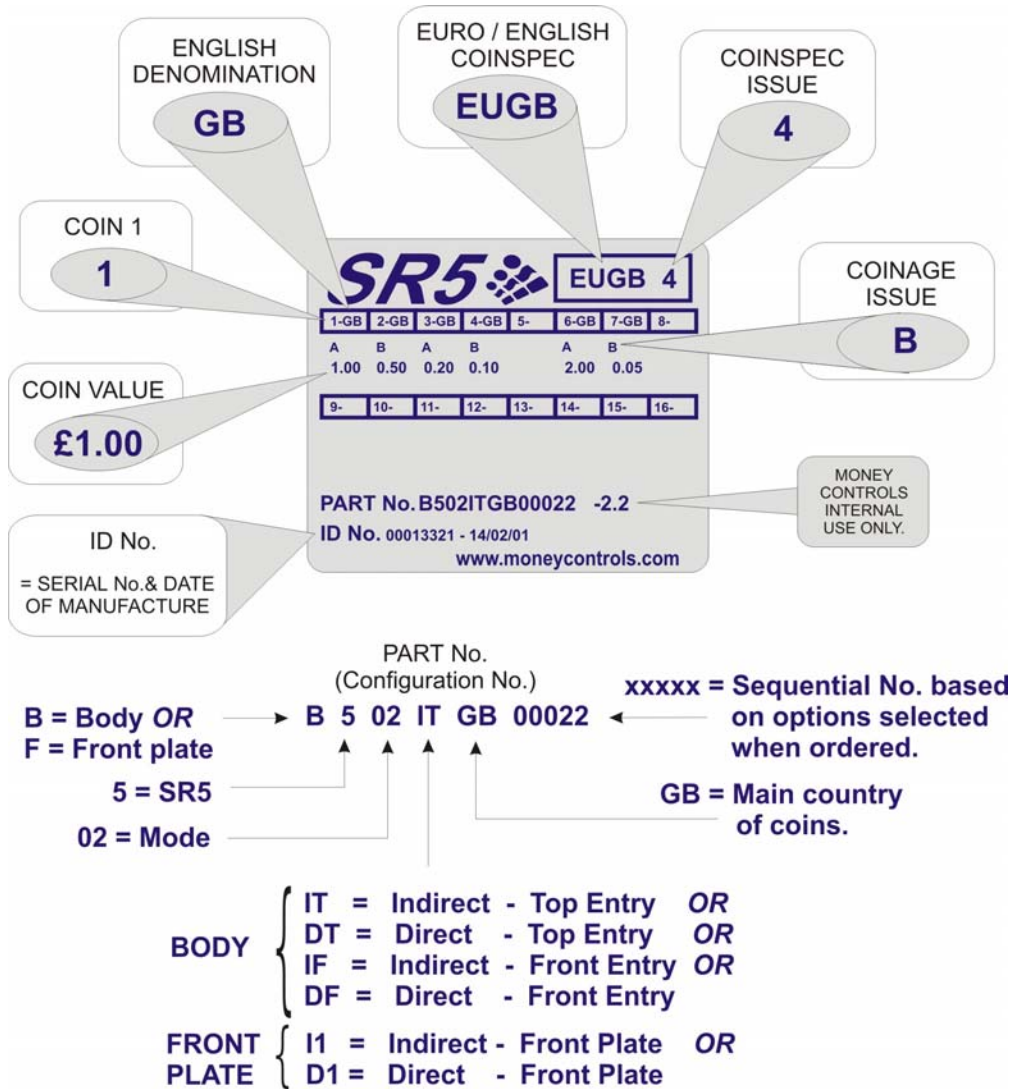
Figure 15: SR5 Label Details
