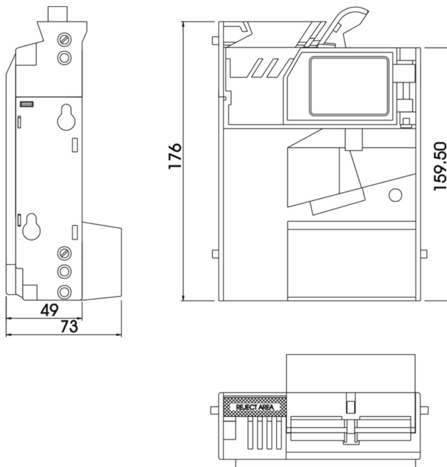
Figure 23: SR5 Top Entry with Sorter Dimensions
