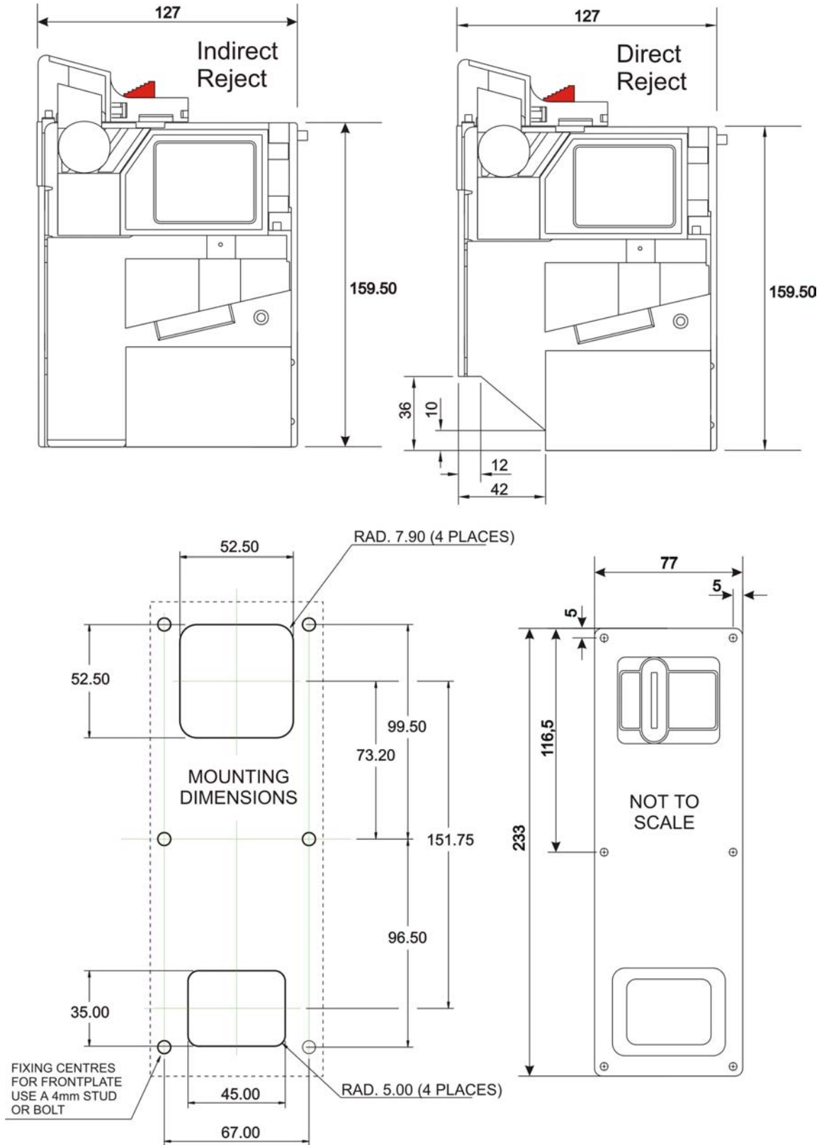
Figure 26: SR5 Front Entry Dimensions
