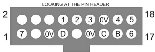
Figure 11: Routing Plug Connections
