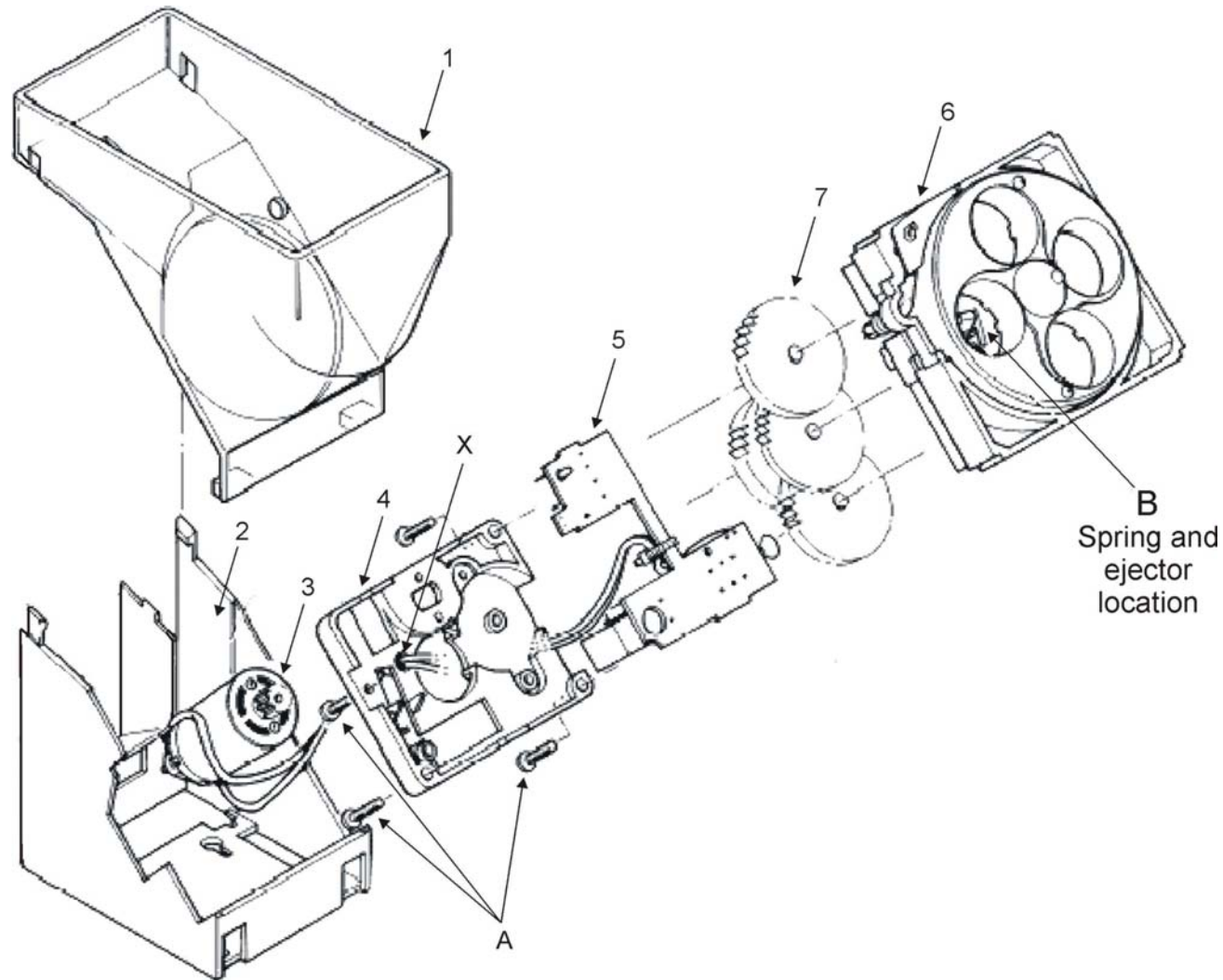
Figure 14: Exploded View
