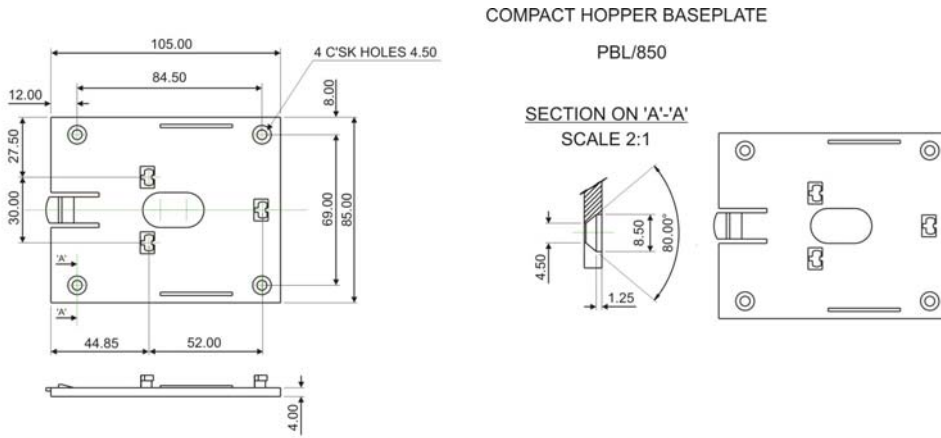
Figure 15: Baseplate Dimensions
