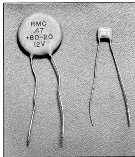
Fig. 1: Both capacitors have the same .47 \mu F value. The disc on the left is only rated at 12 volts, while the monolithic on the right is rated at 50 volts.
