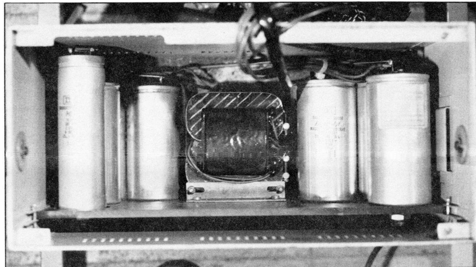
Fig. 7: The capacitors inside a power supply for a flash strobe must quickly charge to relatively high voltages. If one of these capacitors has excessive leakage, it quickly builds up internal pressure from overheating and may explode.
