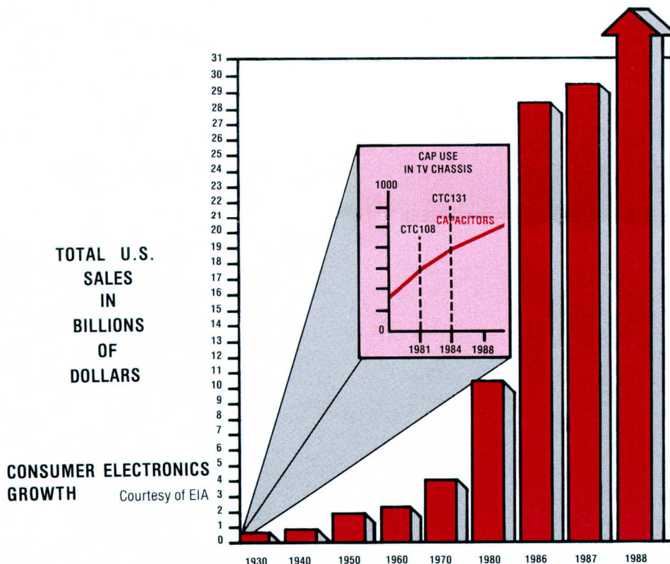
fig. 1: The RCA CTC131 chassis contains 665 capacitors compared to the 1981 CTC108 chassis with only 263 capacitors.
