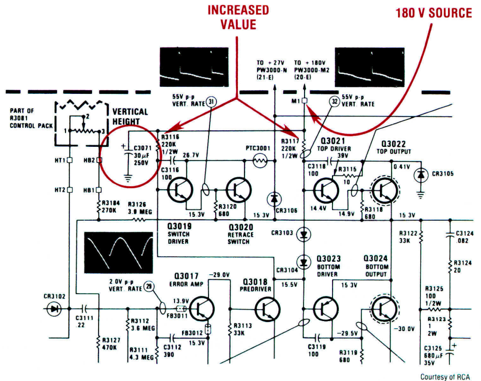
Fig. 3: This schematic shows the vertical output stages of an RCA CTC97 chassis. Even after the defective transistors and bias resistors were replaced, the 180 volt power was low. The problem was traced to a leaky filter cap, C3071.
