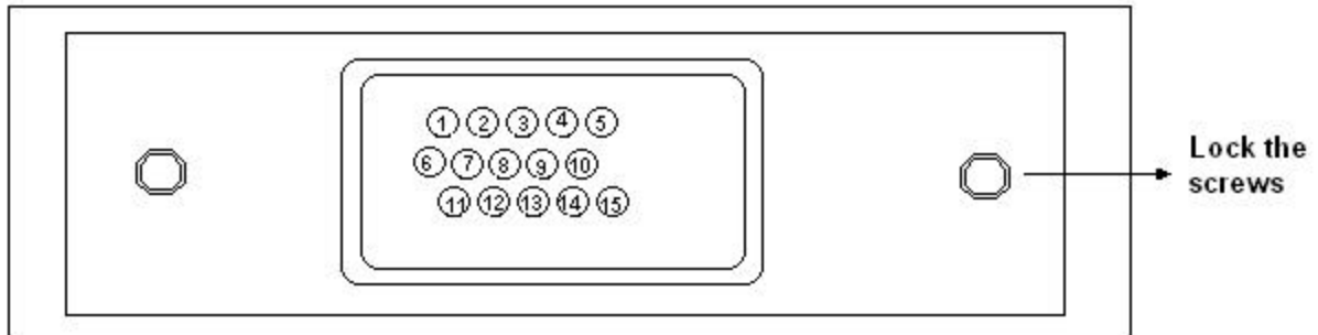
High-density D-type 15pin connector
